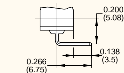
PCB Terminals LH Side with Location Pins 0.024 x 0.020 (0.6 x 0.5)
